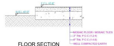
FLOOR SECTION DETAIL
