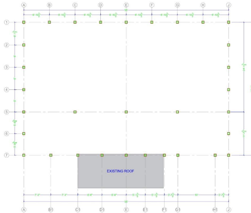
MS COLUMN LAYOUT PLAN
